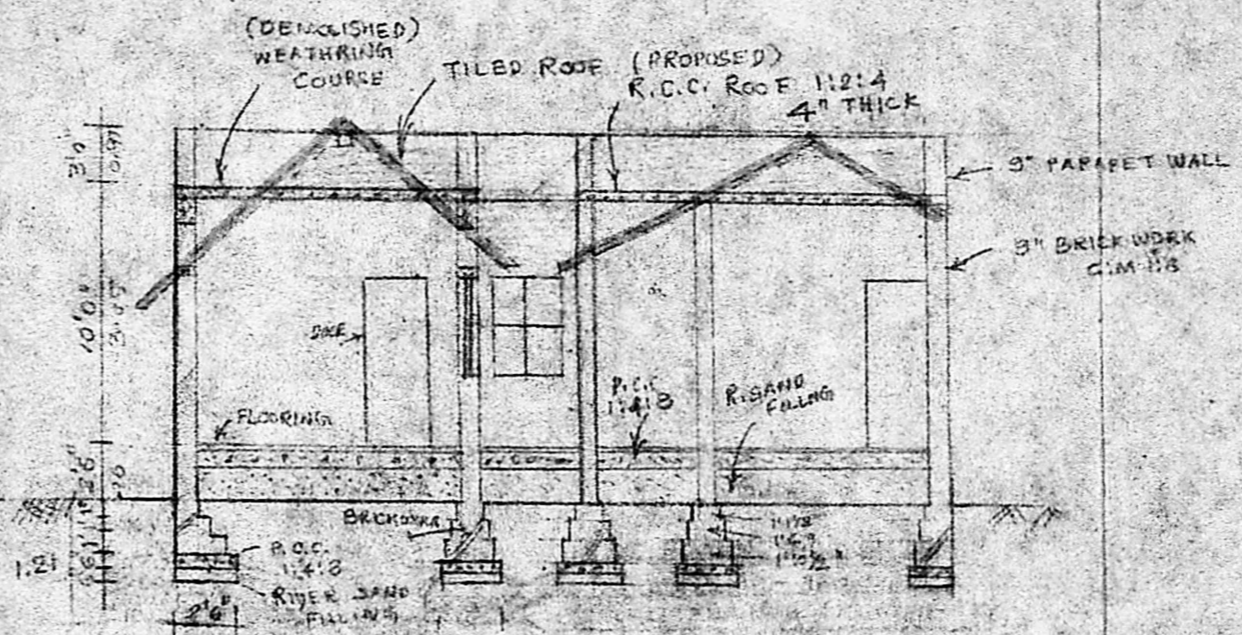
SECTION ON-AA
